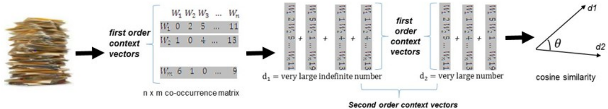
Figure 2: Second-order vector example
